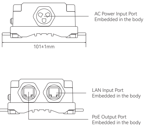
Figure 1-2 Front View Schematic
