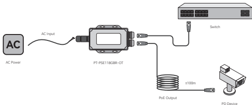
Figure 2-1 Connection Schematic
