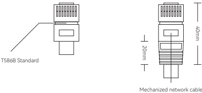
Figure 4-1 Schematic of Common RJ45 Ports
