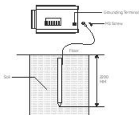
Figure 3-7 Diagram of Simple Grounding Installation
