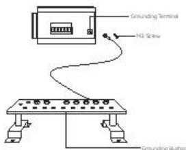
Figure 3-6 Grounding Busbar Installation
