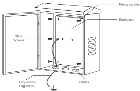
3-2 Installation in waterproof case
