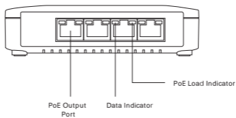
1-3 Front View
